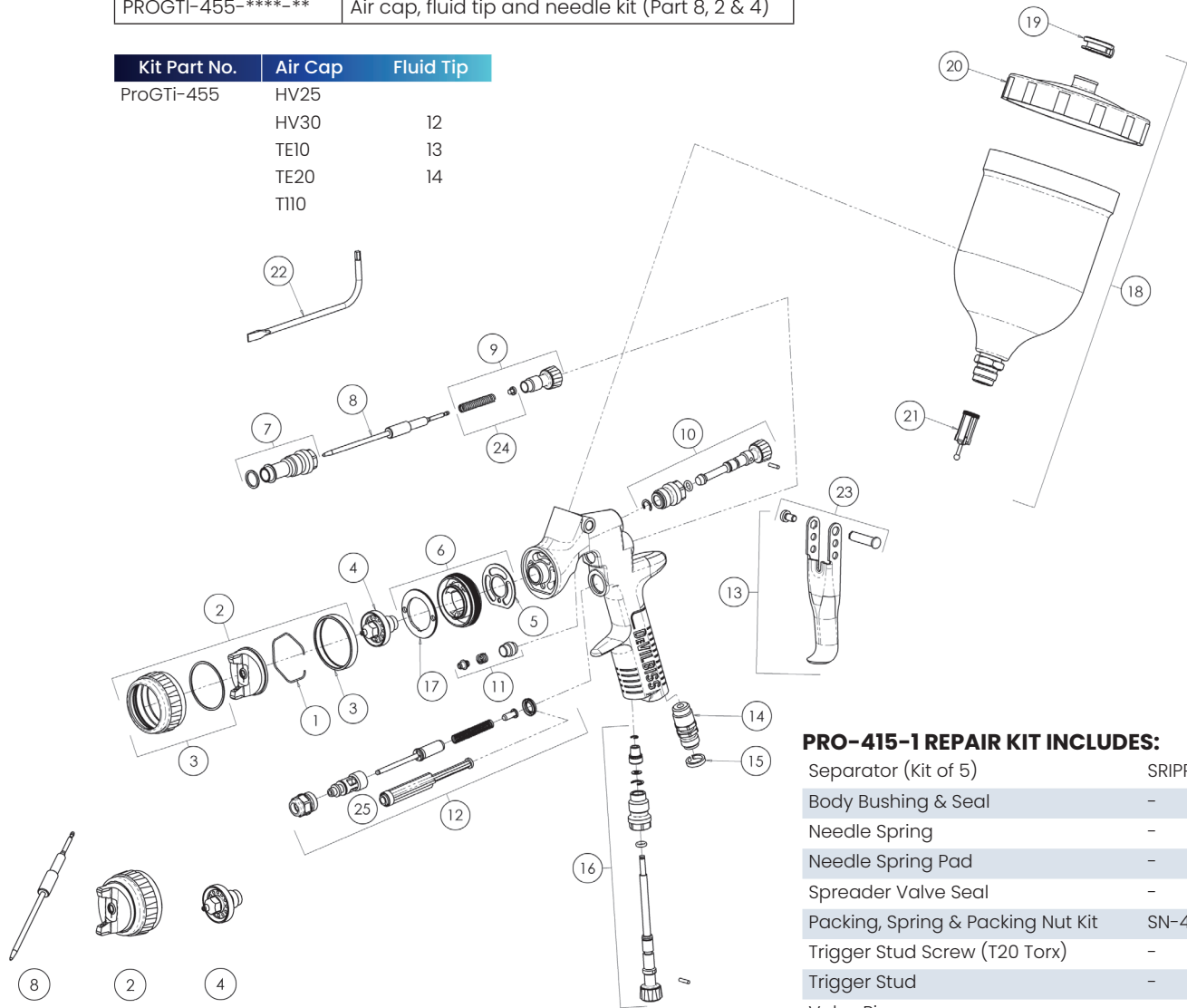
PROGTI-455-****-** Air cap, fluid tip and needle kit (Part 8, 2 & 4)
