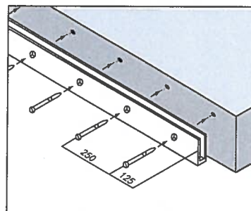
Base Channel For Wall
