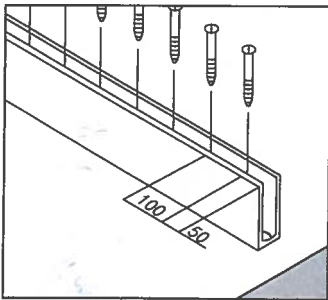
Base Channel For Floor
