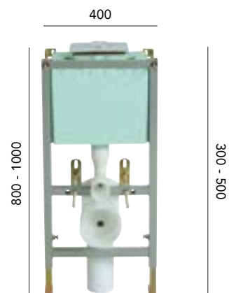
Wall Hung Frame & Concealed Cistern - Top Access
