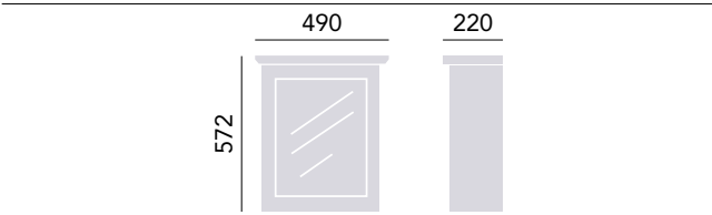
Single Door Mirrored Wall Cabinet White Ash KWA65 £410
