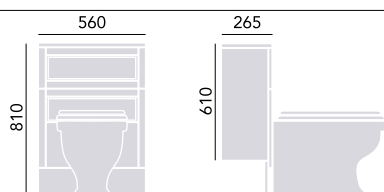
560mm WC Unit
