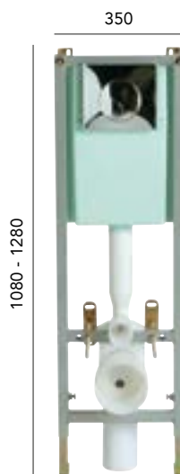
Wall Hung Frame & Concealed Cistern - Front Access
