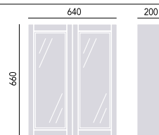
640mm Mirror Wall Cabinet
