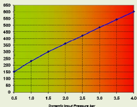
477 Air Cap Air Flow
