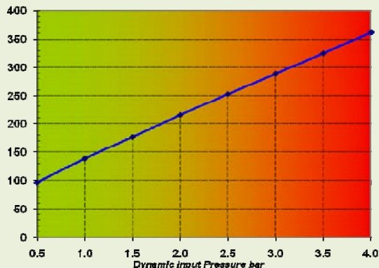
430 Air Cap Air Flow
