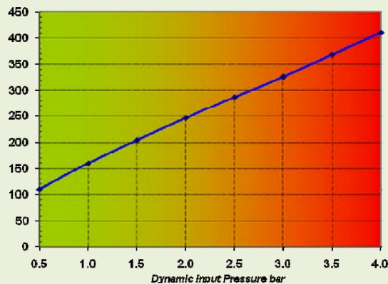
443 Air Cap Air Flow
